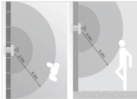
Presence detection area
